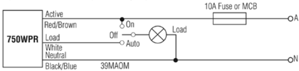
2c) ON, OFF or AUTOMATIC Operation using a 3 position switch
