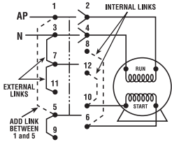
Single Phase Reversing
