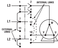
Three Phase Reversing
