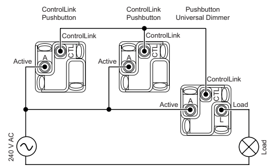
Dimmer Wiring – Three way using x2 ControlLink
