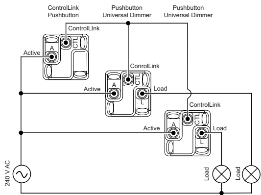
Dimmer Wiring – Three Way using x1 ControlLink
