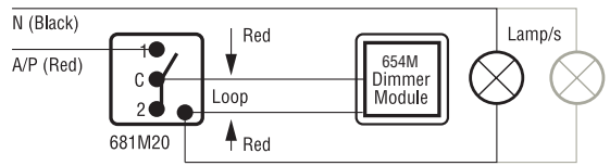
654 Dimmer and 654M Dimmer Module Two way circuit
